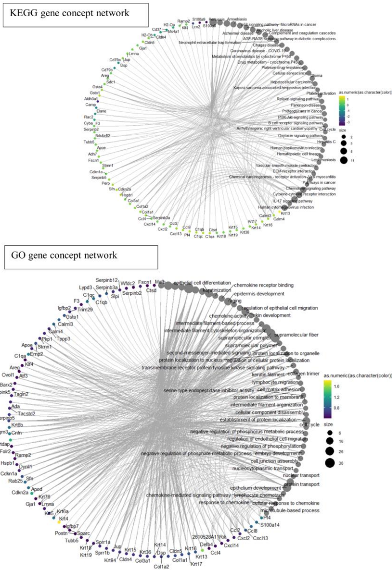
Figure S 5: Gene-concept network of mice senescent cells of the TMS dataset. To determine which genes are involved in the pathways presented in the enrichment map shown in Fig. S4, we need to take into account the fact that a gene may belong to multiple annotation categories, which adds a level of biological complexi-
