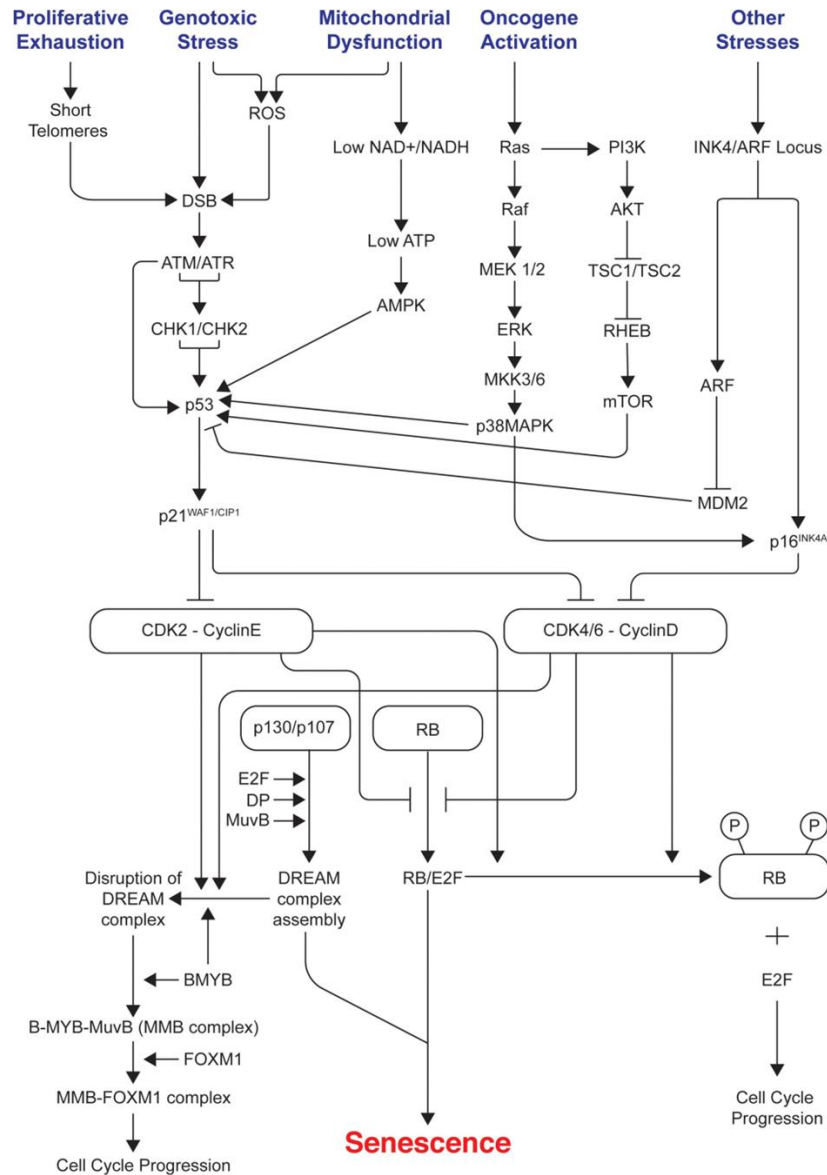
Figure 7: Scheme of signals and pathways involved in mediating senescence cell cycle arrest. The different causes of the senescence state [221].
