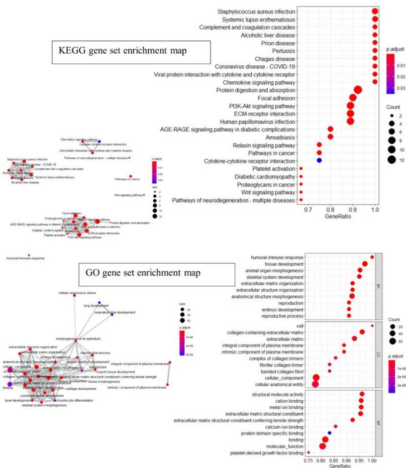
Figure S 9: Dot plots and hypergeometric tests present gene-set enrichment maps of senescent cells from old mice (18-30 months) in the TMS dataset. The findings offer significant insights into the molecular mechanisms that play a role in the aging process and senescence. The KEGG database indicates that the top panel displays the enrichment map of senescent cells from the old mice group, highlighting pathways contributing to inflammation, aging, and age-related diseases. The lower panel demonstrates the expression of the same cell data enrichment, ac-
