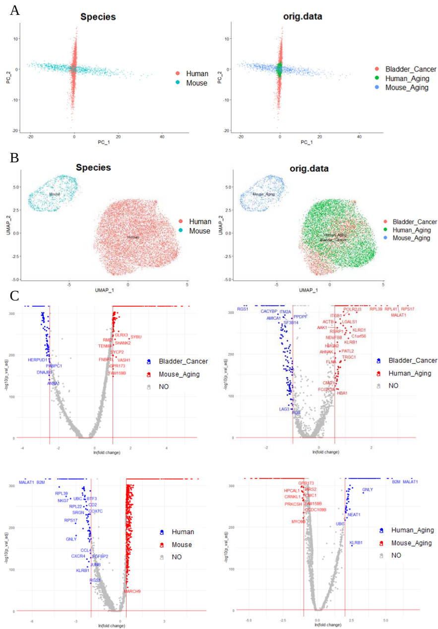
Figure S 1: Comparison of cytotoxic CD4^+ T cells in three datasets: human aging, bladder cancer, and aging mouse datasets. A) The left plot displays the PCA pro-
