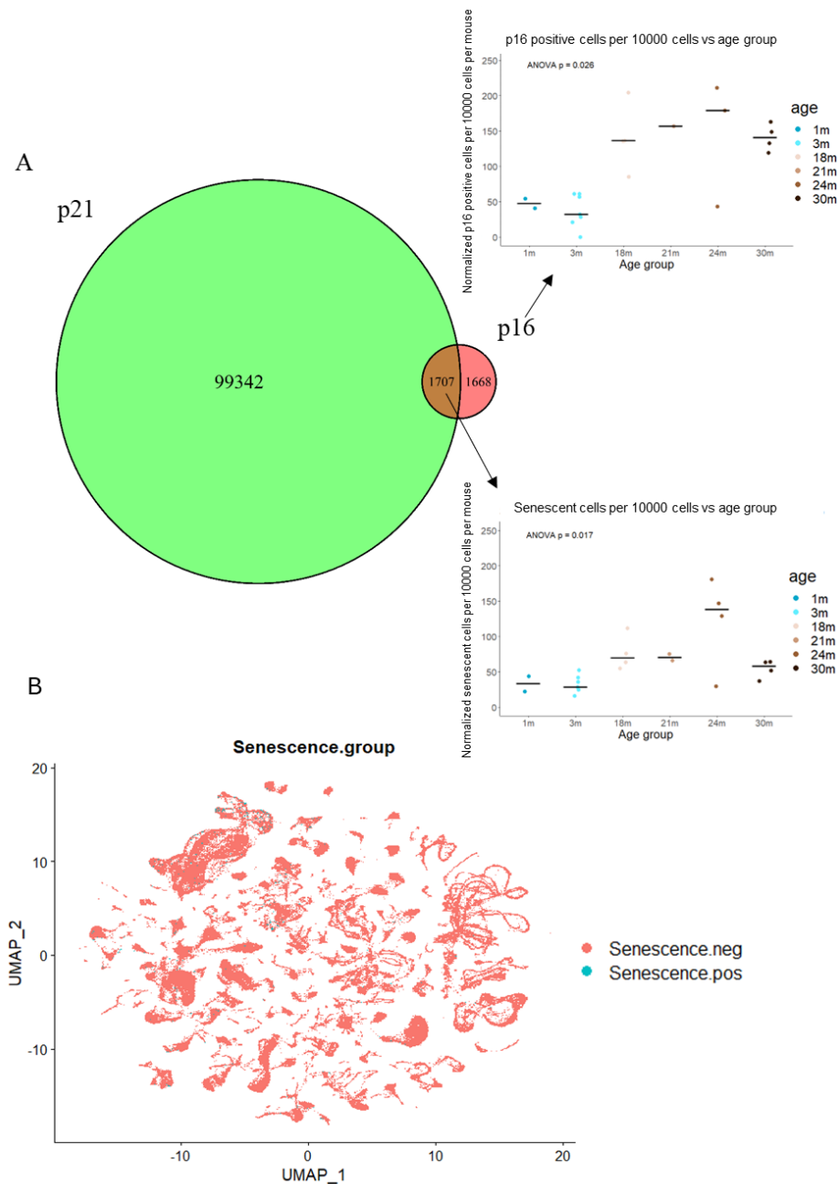
Figure 32: Visualization of senescent cells identification defined by p16^+p21^+ in the TMS dataset. A) Venn diagram displays the overlap of cells expressing p21 (in
