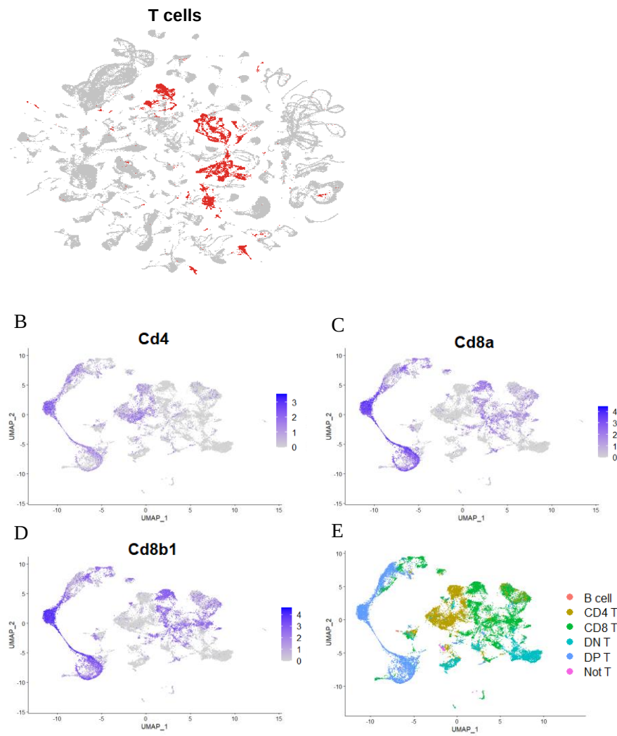
Figure 24: Visualization of T cells in the TMS dataset using UMAP projections. A) Overall distribution of T cells (red) within the total cell population of the TMS dataset; B) UMAP representation highlighting the expression of the CD4 marker in T cells, visualized using a purple scale for gene expression intensity; C-D) UMAP projections showcasing the expression of CD8 markers in T cells, with
