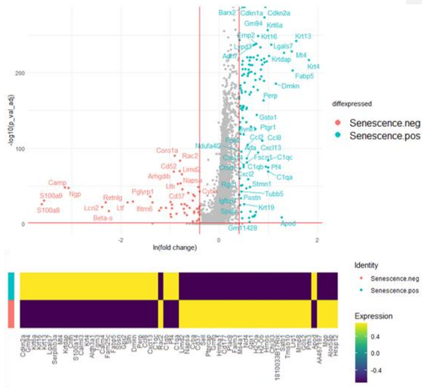
Figure S 3: DGE of senescent cells vs non-senescent cells in the TMS dataset. The volcano plot in the top plane shows the genes that are differentially expressed in
