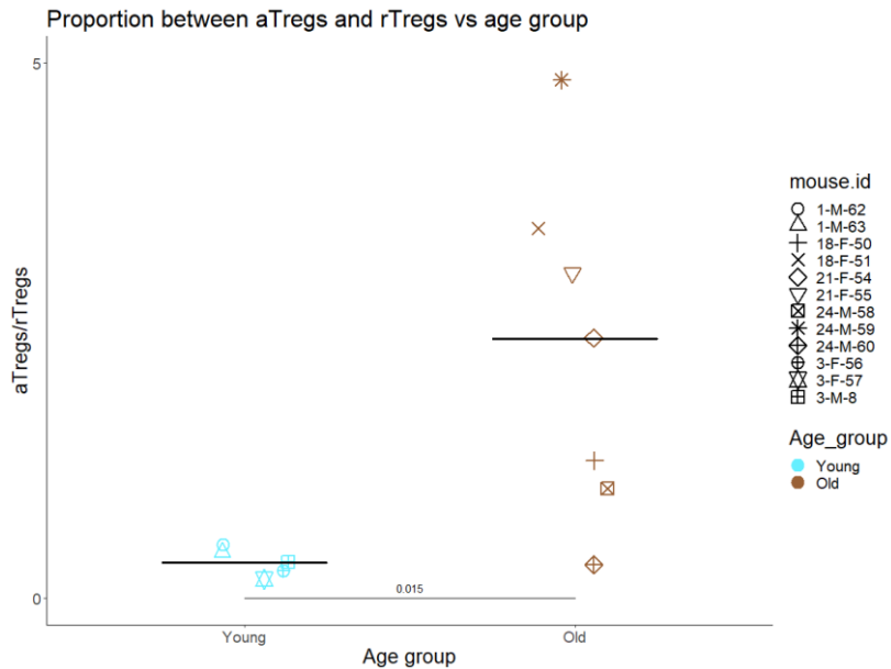
Figure 27: Comparative Analysis of aTregs/rTregs Ratios Across Age Groups in the TMS Dataset. Comparative analysis of the TMS dataset presenting the ratio between aTregs and rTregs across two distinct age groups - young and old. The data points from individual mice are color-coded: the young (light blue) age group and the old (brown) age group. Each mouse within the dataset is uniquely identified with a sign, facilitating a clear delineation of data points between the subjects. Horizontal lines are drawn across the scatter plot to indicate the average ratio of aTregs to rTregs for each age group, providing a visual cue for assessing the central tendency within the dataset concerning the aTregs/rTregs ratio across young and old age groups. Through this graphical representation, the analysis aims to elucidate any significant differences in the aTregs/rTregs ratio that might correlate with aging.
