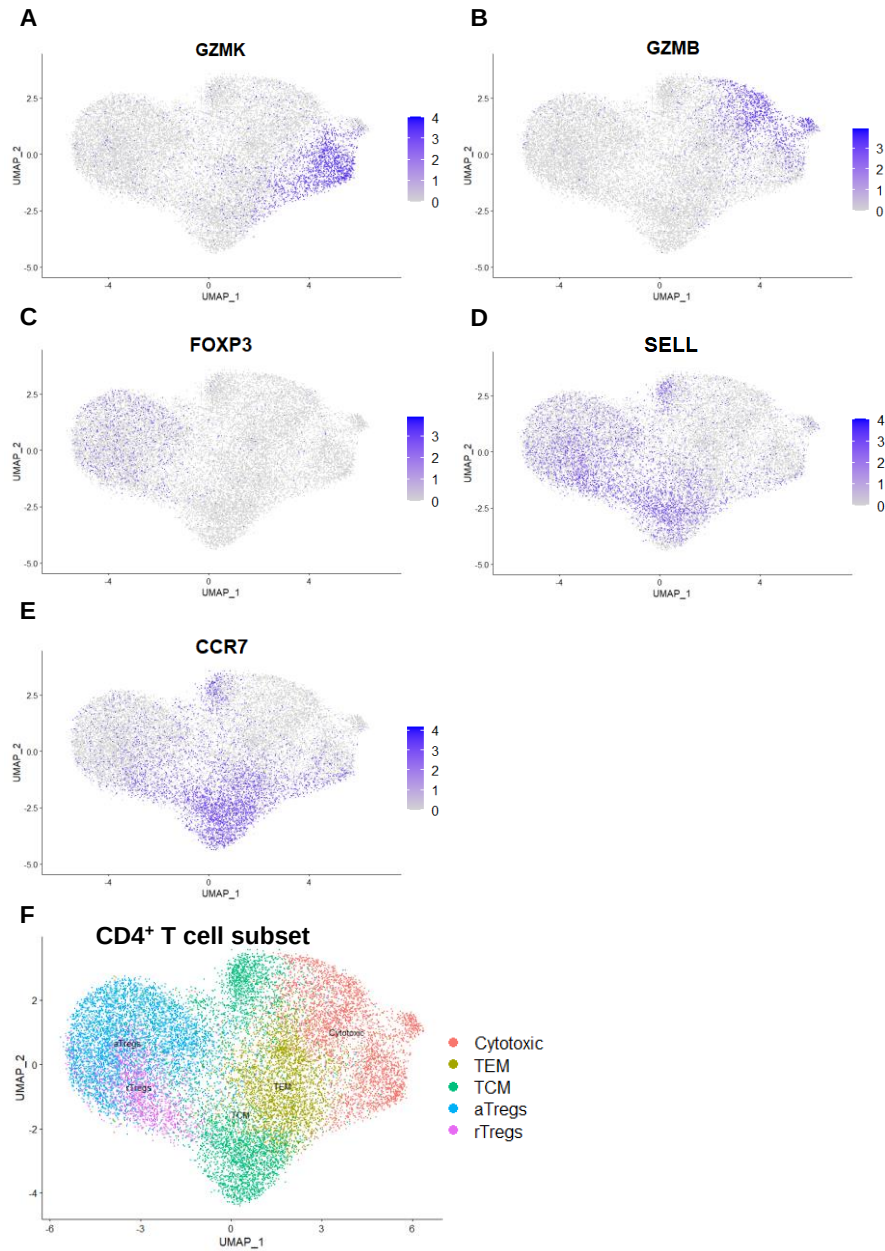
Figure 17: UMAP projection of the CD4 T cells in the bladder cancer dataset. A) UMAP projection of GZMK gene expression; B) UMAP projection of GZMB gene
