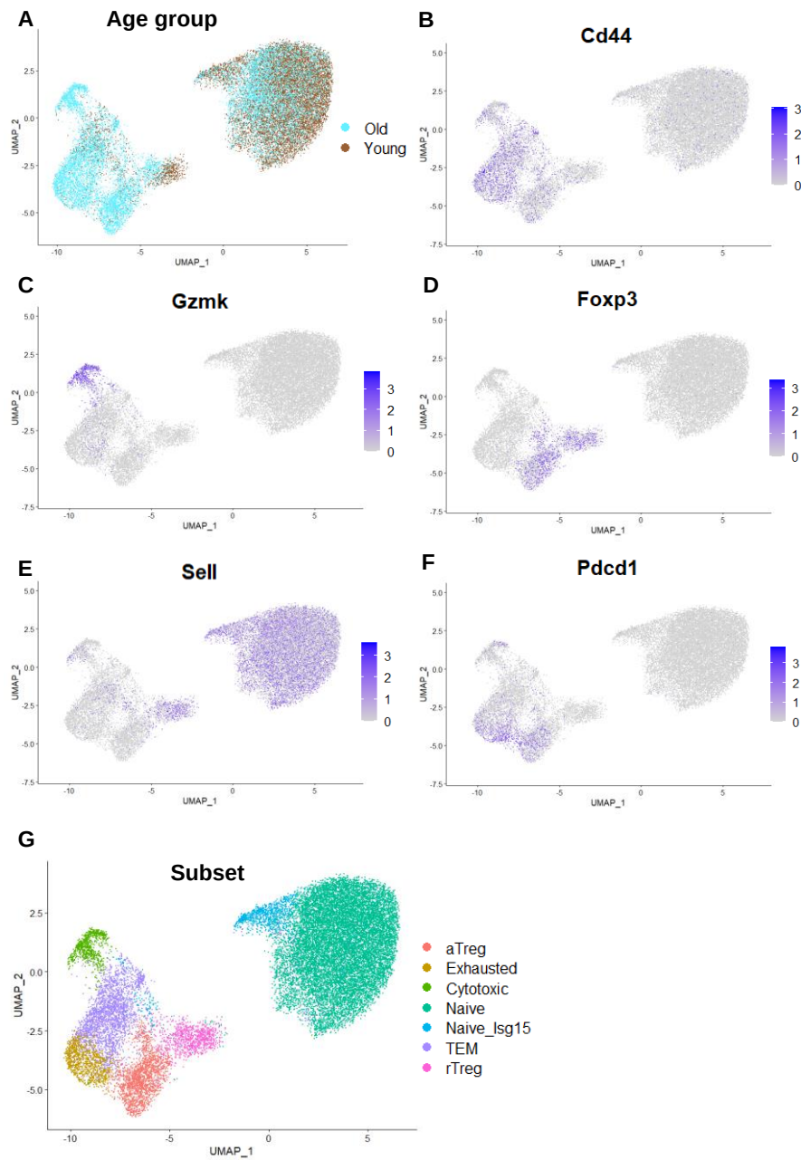
Figure 14: UMAP projection of the CD4^+ T cells of mice in the aging mice dataset grouped by age group and CD4^+ subsets. A) UMAP projection of CD4^+ T
