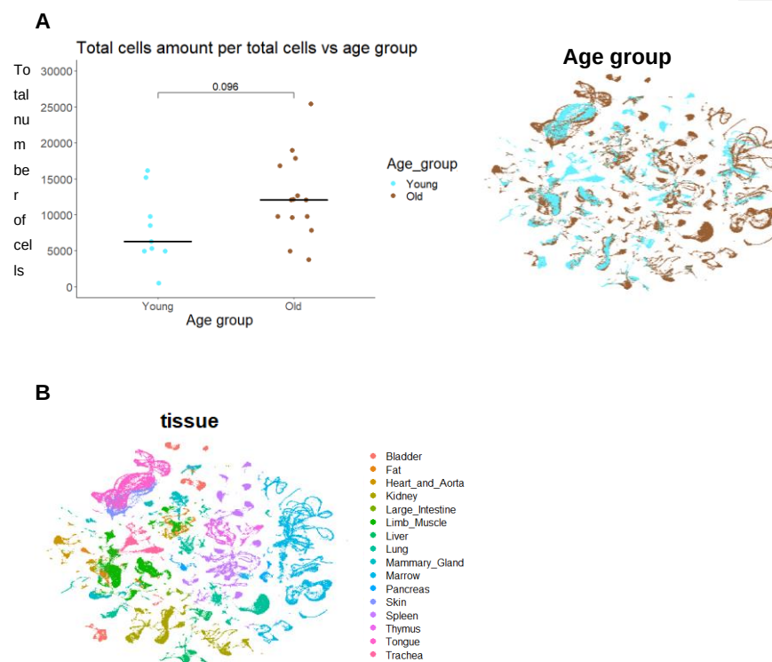
Figure 19: Presentation of TMS Dataset Across Age Groups and Tissue Types. A) Age Group Analysis: Left - Comparative total cell count in young (1-3 months) and old (18-30 months) mice. Right - UMAP projection of total cells by age groups: young (light blue), old (brown). B) Tissue-Specific Distribution: UMAP projection of cells from A Right, grouped by tissues of origin.
