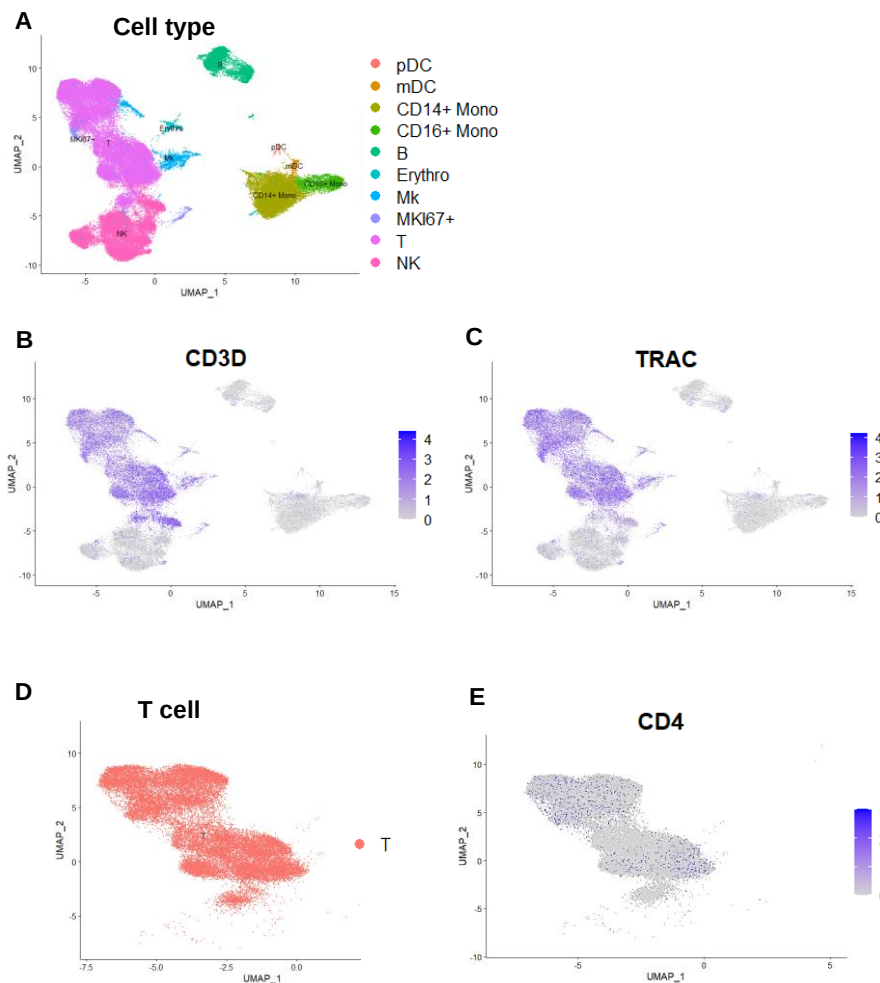
Figure 15: UMAP projections of PBMCs from Hashimoto et al.'s supercentenarian dataset (2019). A) UMAP projection by cell type; B) UMAP projection of CD3D gene expression; C) UMAP projection of TRAC gene expression; D) UMAP projection of T cell subset within PBMC; E) UMAP projection of CD4 gene expression in T cells [93].
